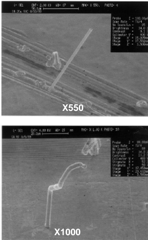
Figure 5. Tin Whiskers on the Non-conformally Coated Side
